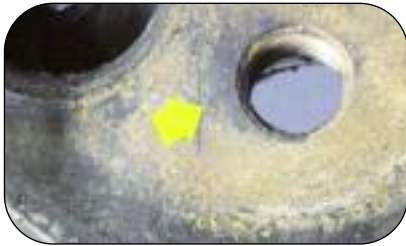
Figure 2 - Damaged Core Refund Bottom deck crack
